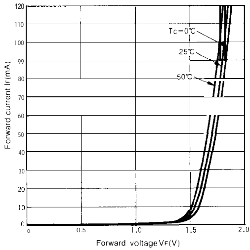
Fig. 77-1 Forward Current vs. Forward Voltage
