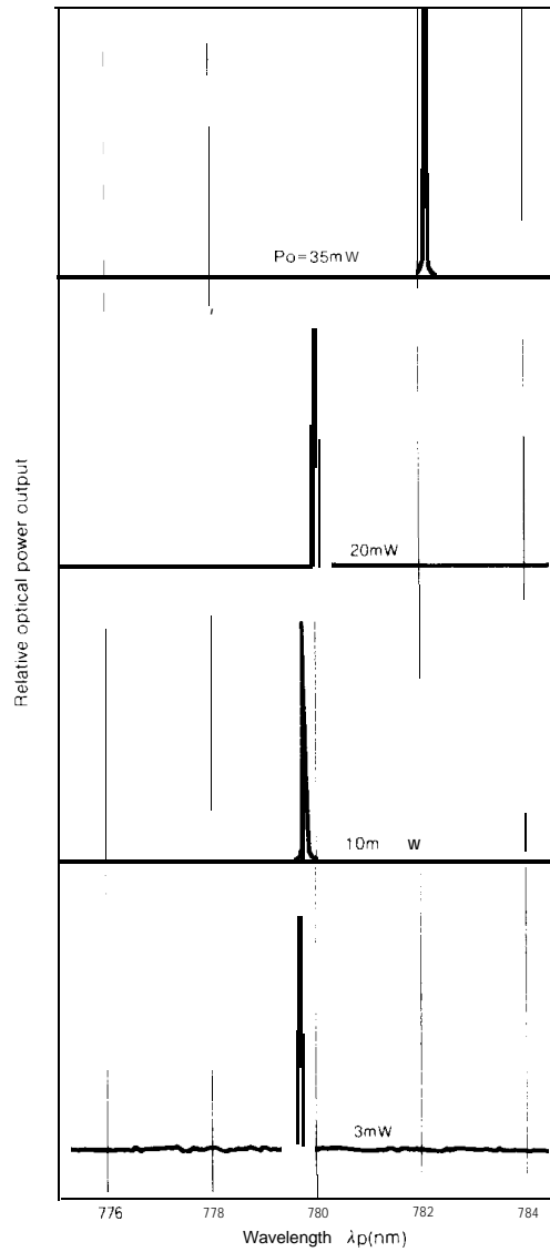
Fig. 77-5 Optical Power Output Dependence of Wavelength
