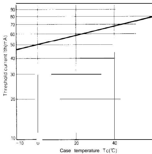
Fig. 77-3 Threshold Current vs. Temperature
